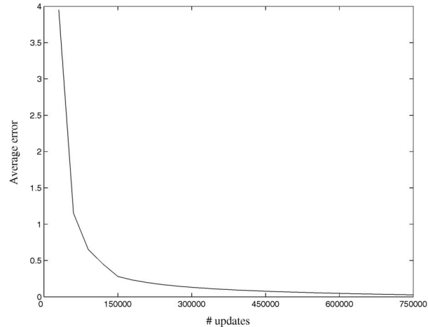
Fig. 2. The average l^2 distance in the RKHS of the first three eigenvectors and their estimates obtained by the KHA. The sign of each PC has been corrected for the computation.
