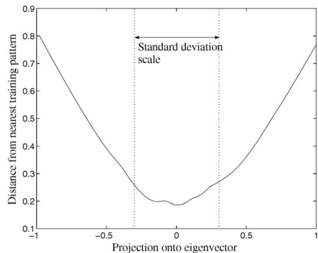
Fig. 8. RKHS distance to the nearest training pattern when moving along the third principal axis.
