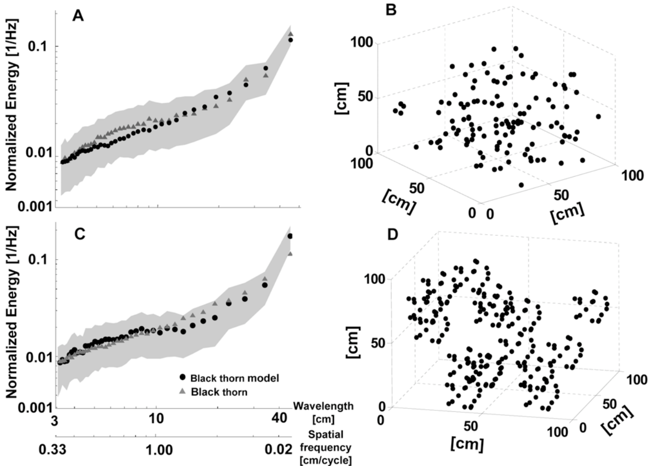
Figure 8. Modeling echo statistics. A) Mean normalized power spectra of blackthorn and the best fitting uniform model for all scales ( d_1 = 16 cm). The shaded area depicts the standard deviation predicted by the model. B) A sample from the uniform 3D Poisson distribution of reflectors with a distance of d = 16 cm. C) Same as A, for the best fitting second-order model ( d_1 = 40 cm, d_2 = 16 cm, r_2 = 50 cm). D) A sample from the 3D distribution of reflectors created by the second-order model with the same parameters as in C. doi:10.1371/journal.pcbi.1000429.g008
