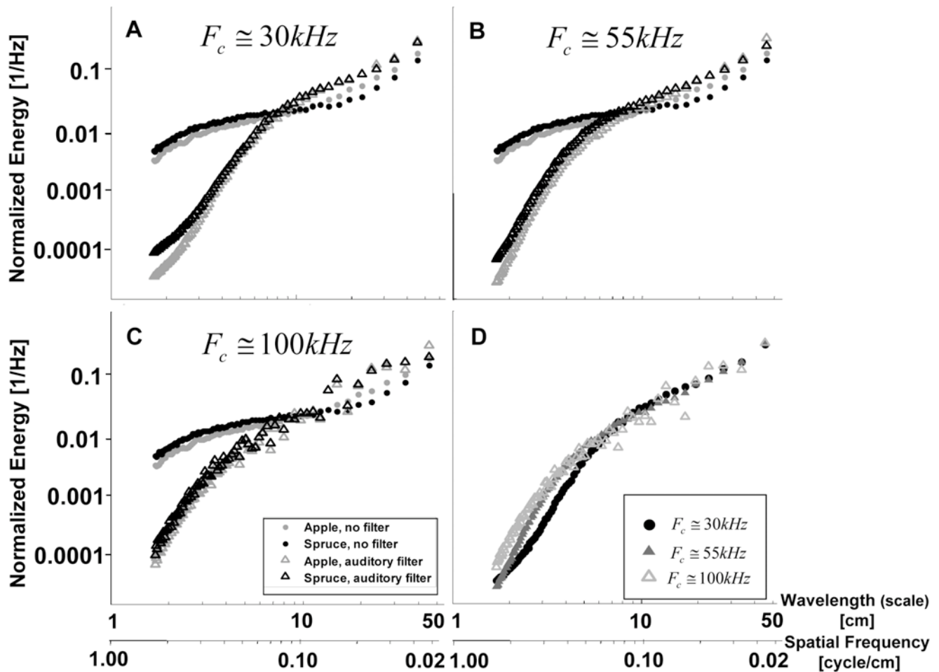
Figure 7. The effect of the auditory system. A–C) Normalized echo spectra of two species (apple and spruce) after auditory system filtering compared to the spectra of the same species with no filtering. The system response is represented by the output of three channels with different center frequencies ( F_c ) representing the entire frequency range. (A) F_c \cong 30kHz , (B) F_c \cong 55kHz , (C) F_c \cong 100kHz . The energy was normalized to a sum of one. D) The output of the three channels of apple (appearing in A–C) are overlaid to emphasize the differences between them. doi:10.1371/journal.pcbi.1000429.g007
