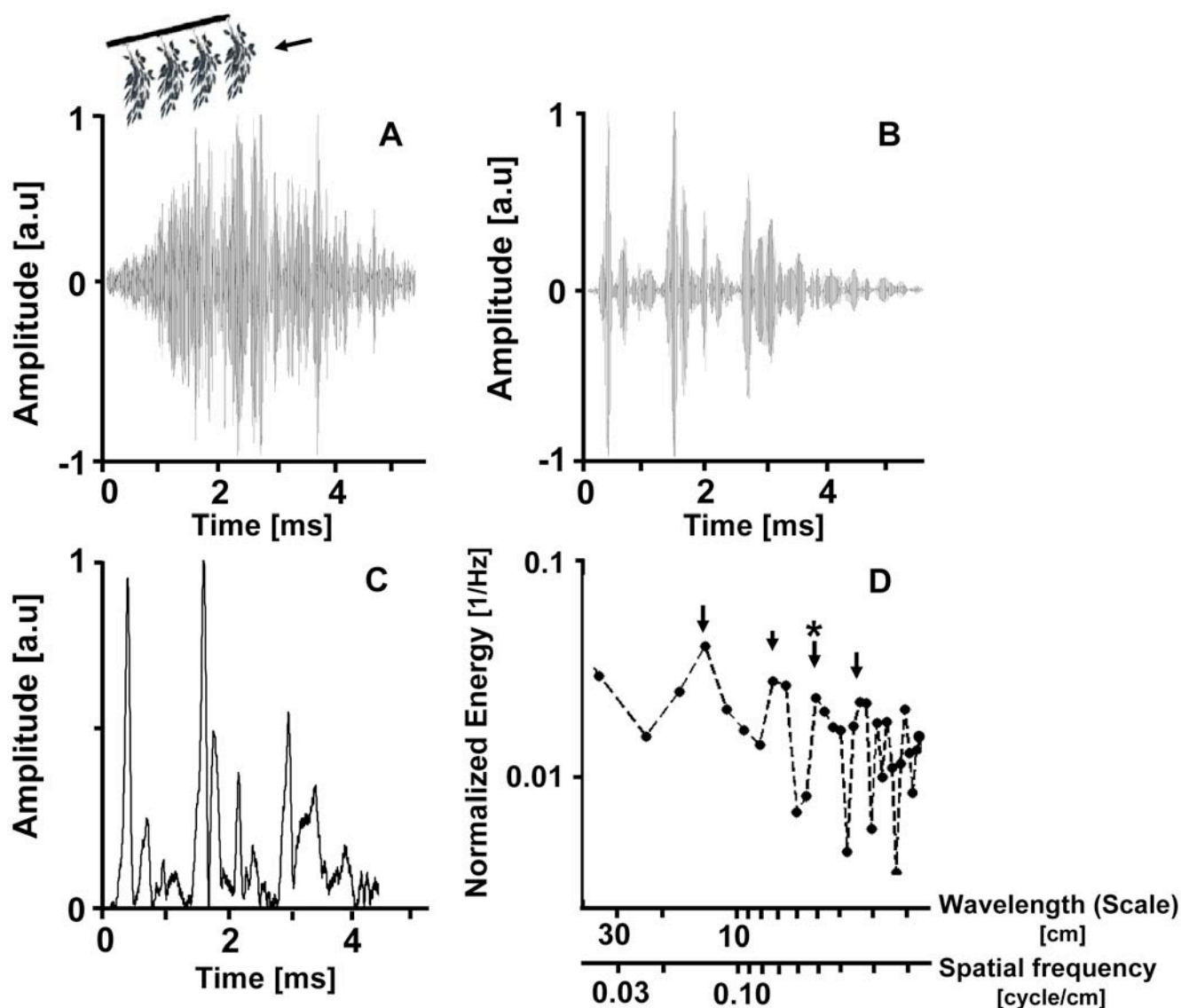
Figure 1. The basic assumption. A) The normalized echo train returning when ensonifying an artificial branch with four identical plastic leaved twigs 15 cm apart from a flat horizontal angle (see illustration above A. a.u. – arbitrary units. B) The normalized IR of the echo train presented in A. C) The normalized envelope of B. Note the clear correspondence to the structure of the plant. The envelope presents three main peaks \sim 0.9 ms apart corresponding to the first three twigs. The echo from the fourth twig is much weaker due to occlusion. Additional smaller peaks follow each of the main ones and correspond to the leaves on the twigs. D) The PSD of C shows a main peak around 14 cm, as expected, with following peaks at the higher harmonics at, e.g., 7, 3.5 and 1.8 cm. One peak however, at \sim 5 cm (marked by an asterisk) deviates from this sequence and is probably a result of the periodic structure created by the leaves on the twigs. The energy (Y-axis) is normalized to a sum of one. doi:10.1371/journal.pcbi.1000429.g001
