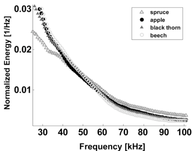
Figure 2. Mean normalized spectra of the echoes. The spectra were first divided by the emitted signal spectrum to calculate the relative reflected energy at each frequency. The result was then normalized to have a sum of one. doi:10.1371/journal.pcbi.1000429.g002
