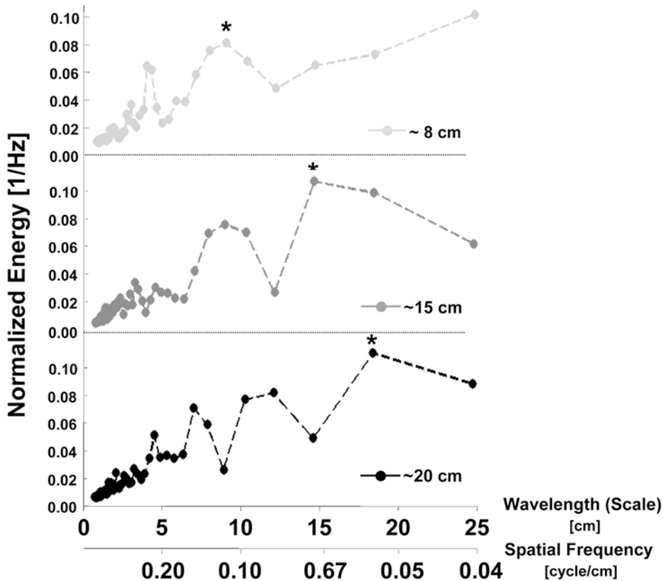
Figure 4. Mean normalized spectra of the envelope of the echo train returning from an artificial branch. Each branch was composed of a row of 4 artificial plastic twigs which were 8, or 15 or 20 cm apart. Notice the energy peaks around 8, 15 and 20 cm in the three graphs (marked with asterisks). Spectra were normalized to have a sum of one. We present the spectra on a linear scale here in order to emphasize the peaks of energy corresponding to the distance between twigs. doi:10.1371/journal.pcbi.1000429.g004
